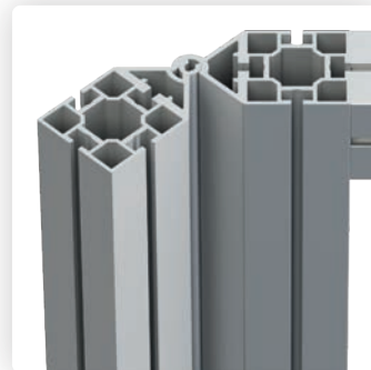
hinge extrusion W 908 for angles between 90° and 180°
