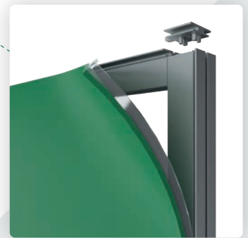
Continuation of the groove with end cap for attaching fabric graphics across frames.
