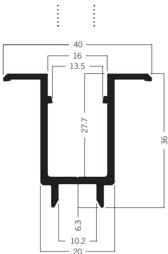
C 210 Clamping extrusion, part B 3.45 kg | 6000 mm
