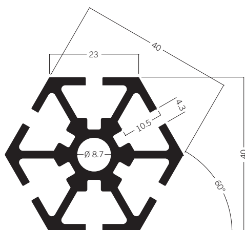
S 500 Upright extrusion 60° 6.98 kg | 5000 mm
