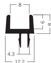
E 422 Glass panel retainer 0.45 kg | 5000 mm
