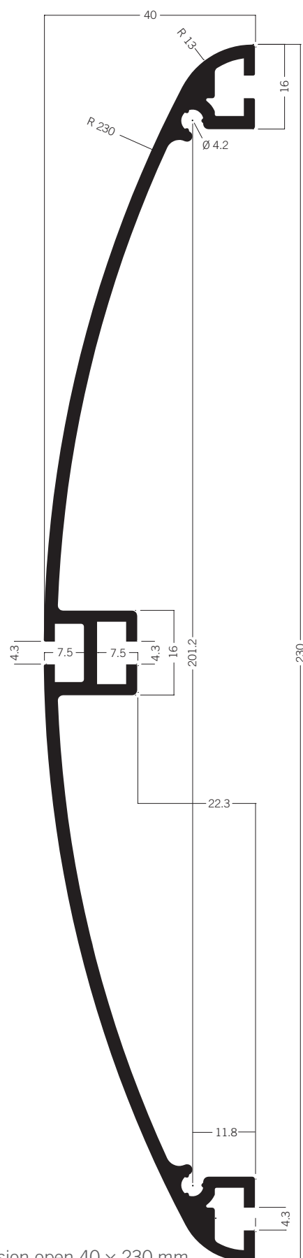
S 2305S* Oval extrusion open 40 x 230 mm 11.55 kg | 5000 mm
