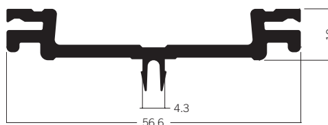
C 159 Adaptor extrusion 10 x 55.5 mm 2.04 kg | 6000 mm
