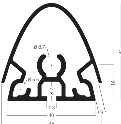
M 1502 Louver extrusion 5.59 kg | 5000 mm
