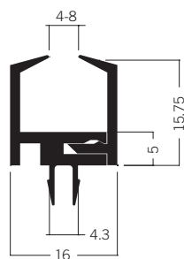
E 420 Glass panel retainer 0.83 kg | 5000 mm
