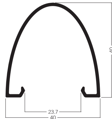
M 1483 Oval cover extrusion 40 mm 2.15 kg | 5000 mm
