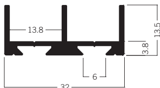
E 470/N Sliding door extrusion 1.74 kg | 5000 mm
