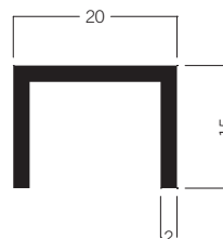
M 1312 U-channel extrusion 1.56 kg | 6000 mm
