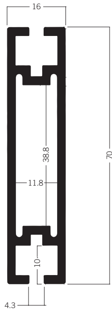
Z 110 Beam extrusion 70 mm 5.42 kg | 5000 mm
