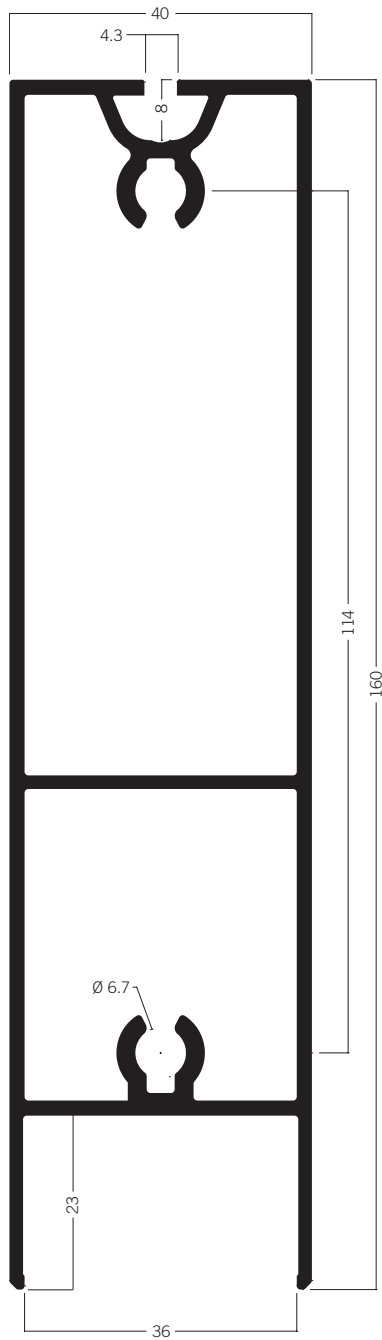
C 315 Door beam extrusion 40 × 160 mm 16.36 kg | 6000 mm
