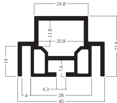
W 903 T-connction extrusion 4.59 kg | 5000 mm
