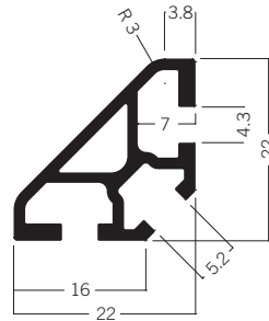
M 1622 Triangular extrusion 1.77 kg | 5000 mm
