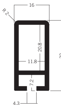
Z 303 Beam extrusion 32 mm 2.70 kg | 5000 mm
