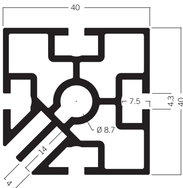
S 382 Upright extrusion, with silicone edge groove 6.91 kg | 5000 mm
