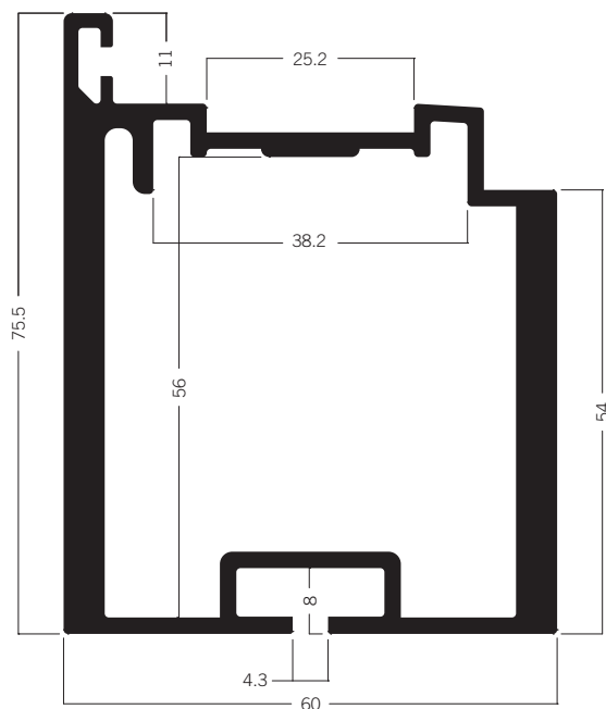
C 309 Door panel extrusion 60 × 75.5 mm 14.46 kg | 5500 mm
