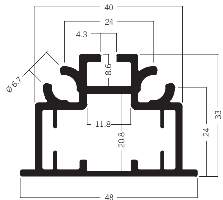
S 1610 Frame extrusion 48 mm 6.48 kg | 6000 mm
