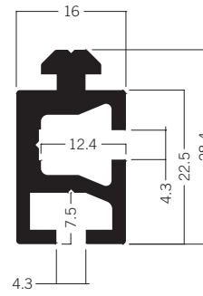
S 204 Wall insert extrusion 2.98 kg | 5000 mm
