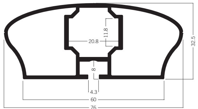
DFL 400A* Handrail extrusion 7.12 kg | 6000 mm
