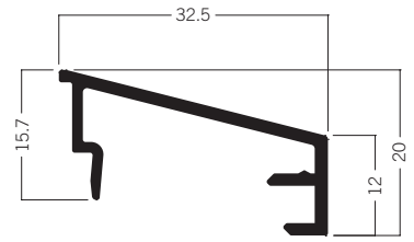
C 171 Retainer extrusion, horizontal 1.64 kg | 6000 mm
