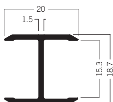
C 630 H-extrusion 20 x 19 mm 1.28 kg | 6000 mm
