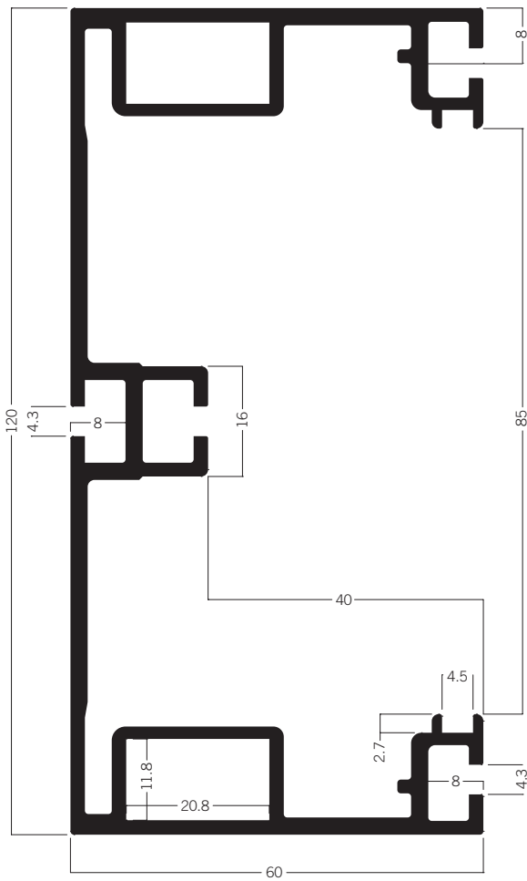
M 1060 Rectangular extrusion open 120 mm 12.94 kg | 5000 mm
