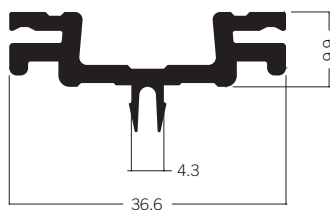
C 160 Adaptor extrusion 10 x 36.6 mm 1.61 kg | 6000 mm
