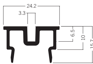
C 153 Spacer extrusion 1.69 kg | 6000 mm
