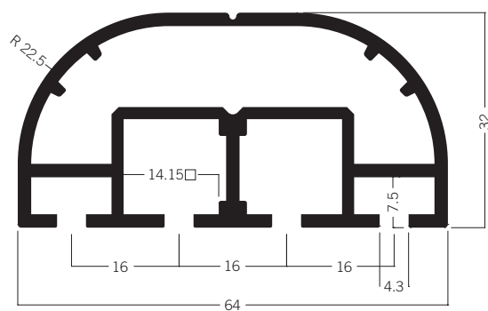
S 1106 Semi-circular extrusion 6.98 kg | 5000 mm
