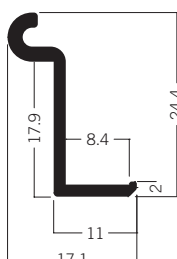
C 612 Support extrusion 17 x 24 mm 1.11 kg | 6000 mm
