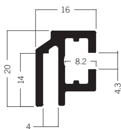
M 1601 Tension fabric extrusion 20 mm 2.16 kg | 6000 mm
