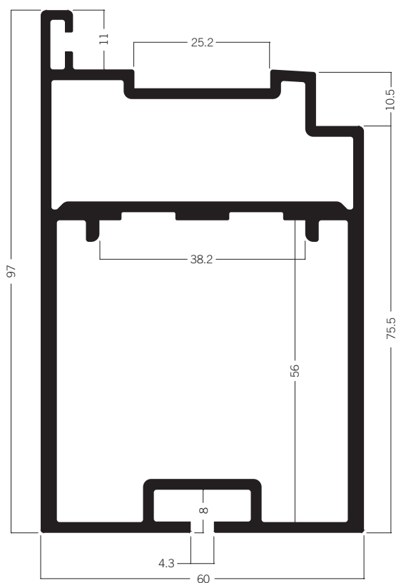
C 311 Double door panel extrusion 60 × 97 mm 9.09 kg | 6000 mm
