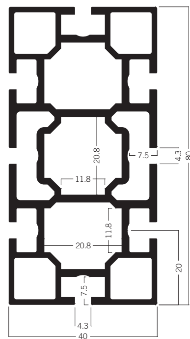
M 1091 Rectangular extrusion 80 mm 12.16 kg | 5000 mm
