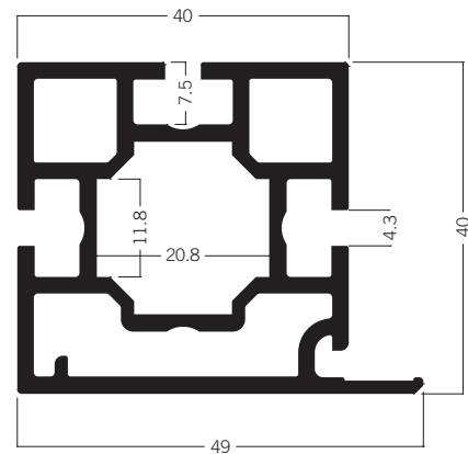
C 701 Extrusion 40 × 49 mm 8.88 kg | 6000 mm
