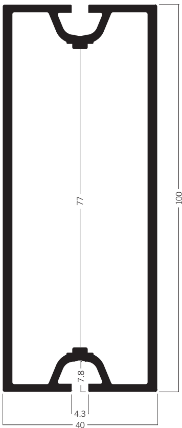
M 1029 Rectangular extrusion 100 mm 11.88 kg | 6000 mm
