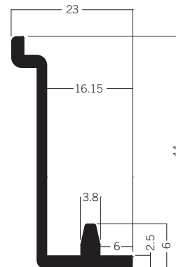
M 1581 Wall panel retainer, bottom 2.02 kg | 5000 mm
