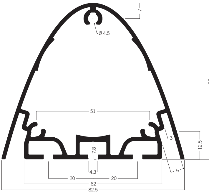
S 3050 Oval extrusion 11.34 kg | 6000 mm
