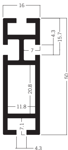
Z 460 Beam extrusion 50 mm 3.96 kg | 5000 mm
