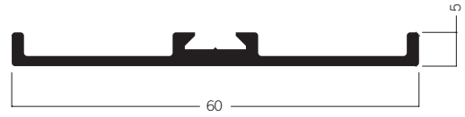
W 810 Cover extrusion 60 mm 1.77 kg | 5000 mm
