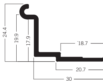
C 613 Support extrusion, wide 1.82 kg | 6000 mm
