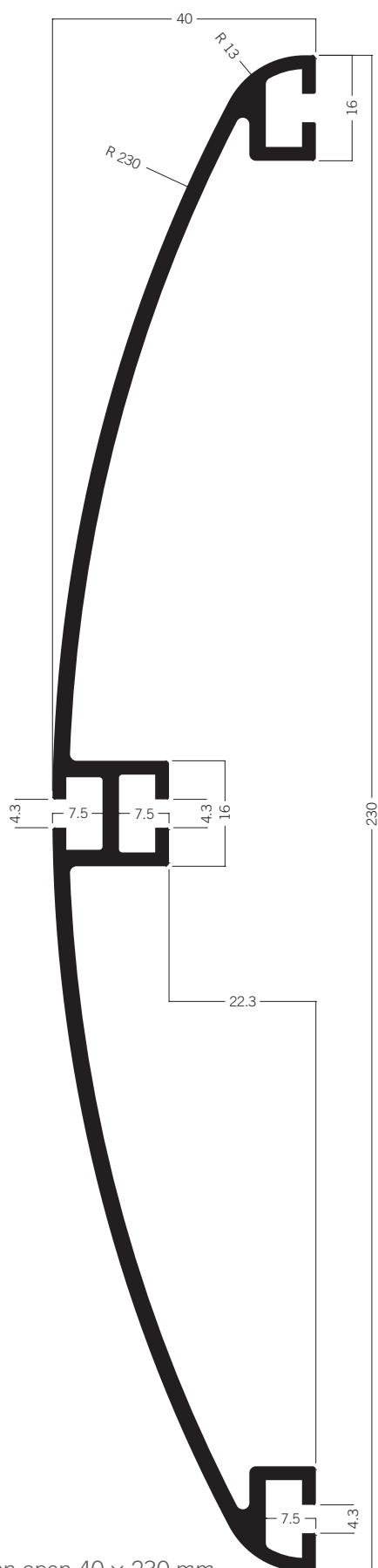
S 2305 Oval extrusion open 40 x 230 mm 11.53 kg | 5000 mm
