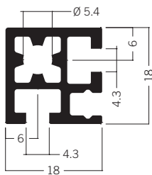
M 1618 Square extrusion 18 mm 1.99 kg | 5000 mm
