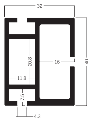
Z 2105 Beam extrusion 40 mm 5.56 kg | 5000 mm
