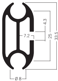
M 1324 Fabric suspension extrusion 33.5 mm 2.58 kg | 5000 mm
