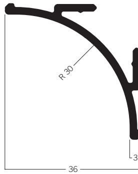
C 1301 Channeling extrusion 36 × 36 mm 2.62 kg | 6000 mm
