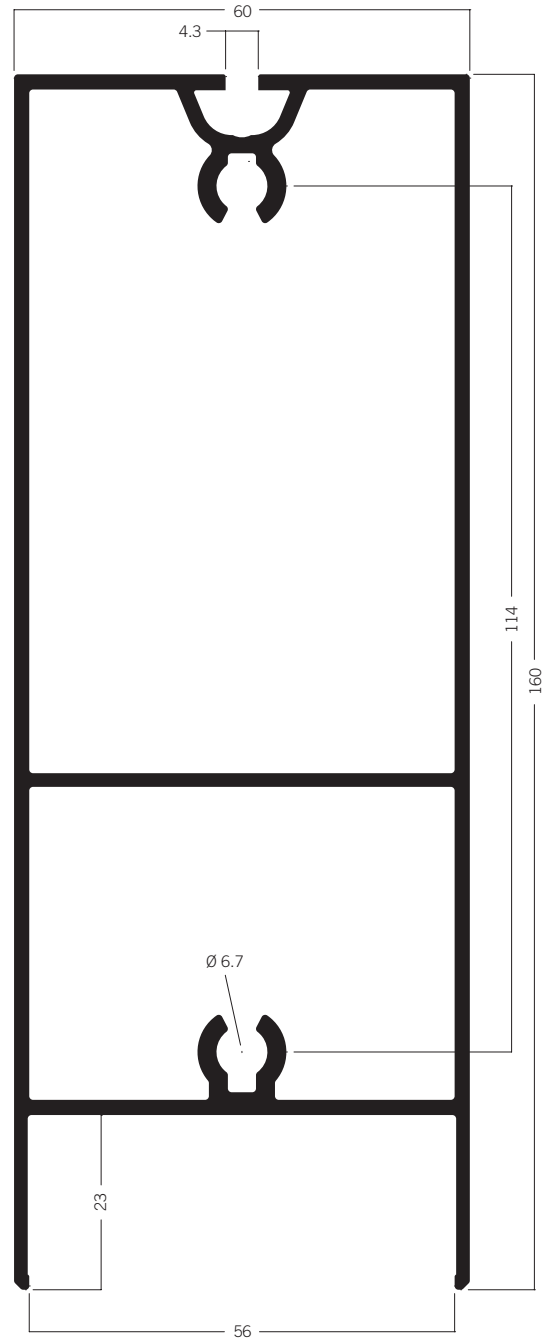
C 316 Door beam extrusion 60 × 160 mm 18.12 kg | 6000 mm
