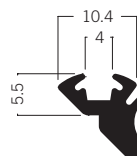
E 445 Anti-rattle strip 3.50 kg | 50000 mm
