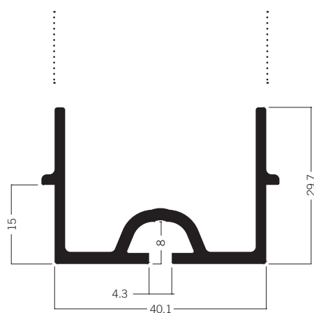
M 1059 Light track mounting extrusion 80 mm 15.92 kg | 6000 mm
