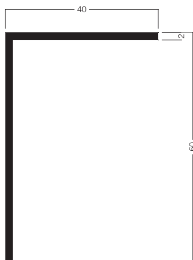
C 680 L-extrusion 60 x 40 mm 2.96 kg | 6000 mm
