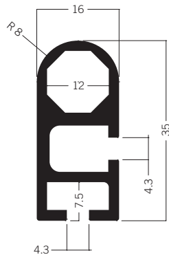
S 250 Hinged extrusion 35 mm 3.14 kg | 5000 mm
