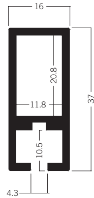
Z 310 Beam extrusion 37 mm 2.96 kg | 5000 mm
