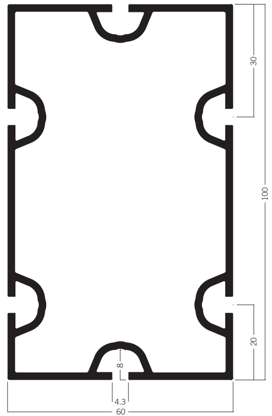
C 1050 Upright extrusion 60 × 100 mm 13.94 kg | 6000 mm
