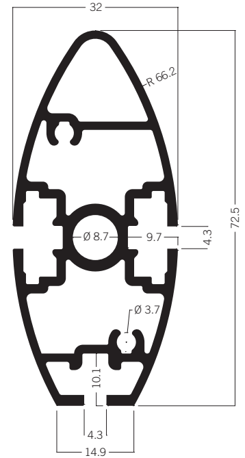
S 6105 Oval extrusion 32 x 72.5 mm 7.65 kg | 5000 mm
