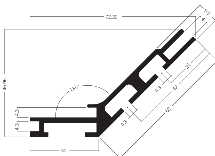
M 1614 Tension fabric extrusion 28 mm 1.54 kg | 6000 mm
