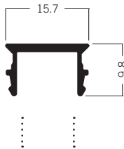
C 220 Cover for clamping extrusion, part B 0.68 kg | 6000 mm
