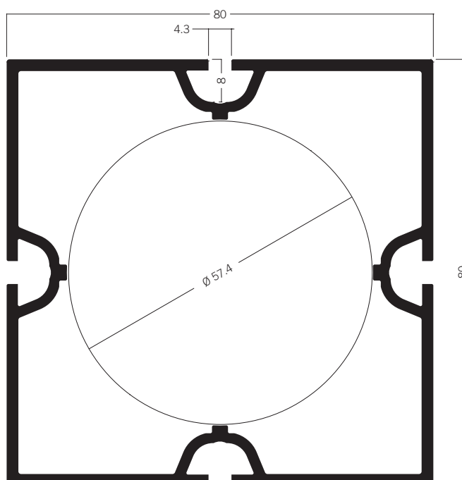
M 1020 Square extrusion 80 mm 11.51 kg | 5000 mm
