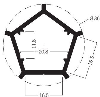
M 1980 Light element extrusion 2.65 kg | 5000 mm
