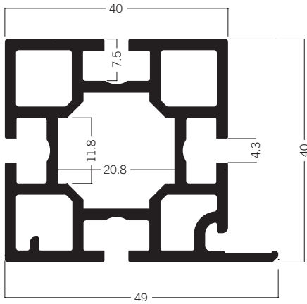
C 604 Extrusion 40 × 49 mm 9.15 kg | 6000 mm
