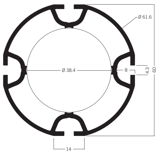
M 1210 Round extrusion 60 mm 6.76 kg | 5000 mm
