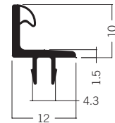
E 433 Door stopping extrusion 0.32 kg | 5000 mm
